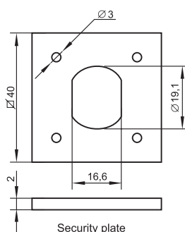
Security plate
